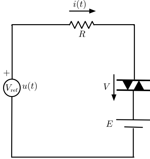
Figure 5.2: A DIAC Clipping circuit
