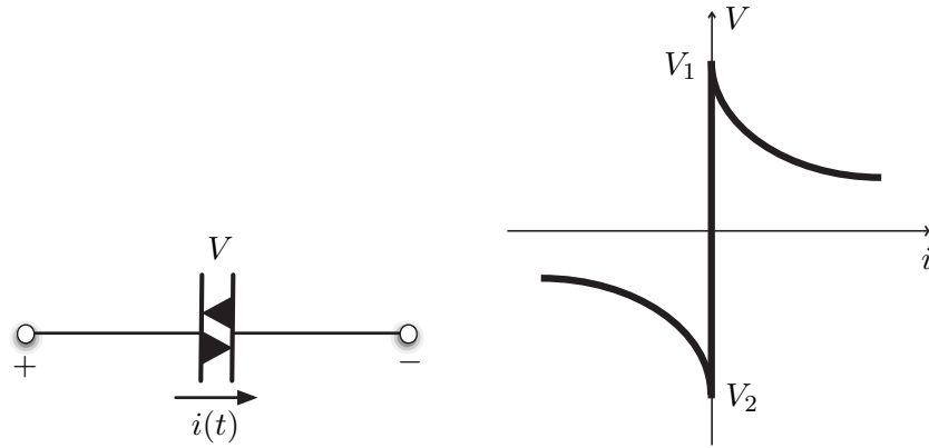
Figure 5.1: I-V characteristic of a DIAC
