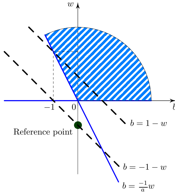
Figure 5.3: Lipschitz modulus of a DIAC
