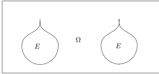
Figure 4.3: u = \mathbb{1}_E \in BV(\Omega)
