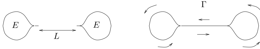
Figure 3.2: The curve \Gamma is canonically associated with the representation of \overline{F}(\mathbf{1}_E)
