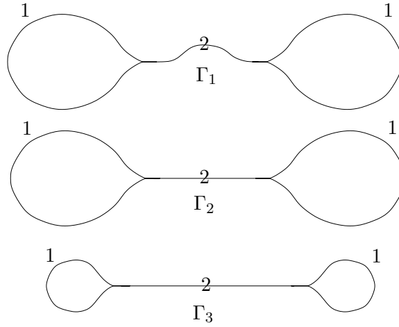
Figure 2.5: The systems \Gamma_1, \Gamma_2, \Gamma_3 with their multiplicities
