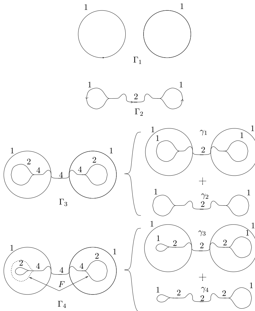
Figure 2.3: The systems \Gamma_1, \Gamma_2, \Gamma_3, \Gamma_4 with their multiplicities
