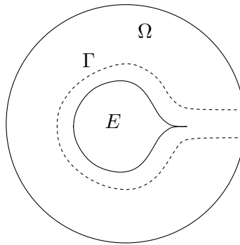
Figure 4.1: \overline{F}(\mathbb{1}_E) = \infty but \overline{F}_B(\mathbb{1}_E, \Omega) < \infty
