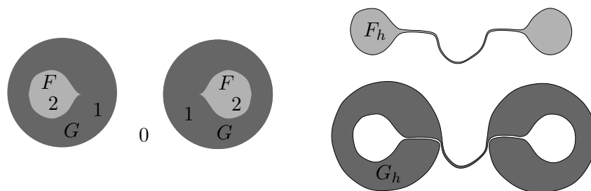
Figure 1.3: The sets G and F can be simultaneously approximated without violating the noncrossing condition
