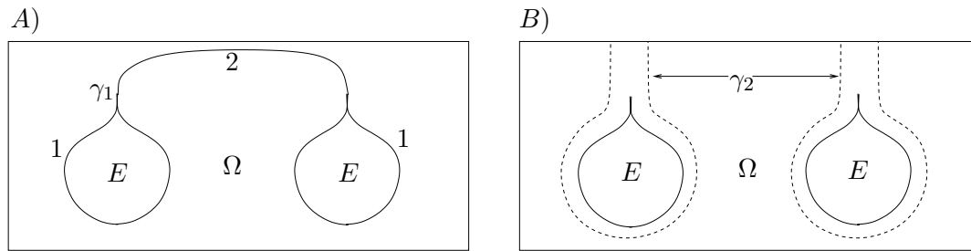
Figure 4.4: Relaxation using sequences belonging to C_c^2(\Omega) (left) or C^2(\Omega) (right)
