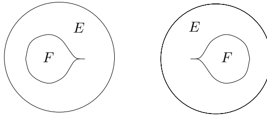
Figure 2.2: Level sets of u
