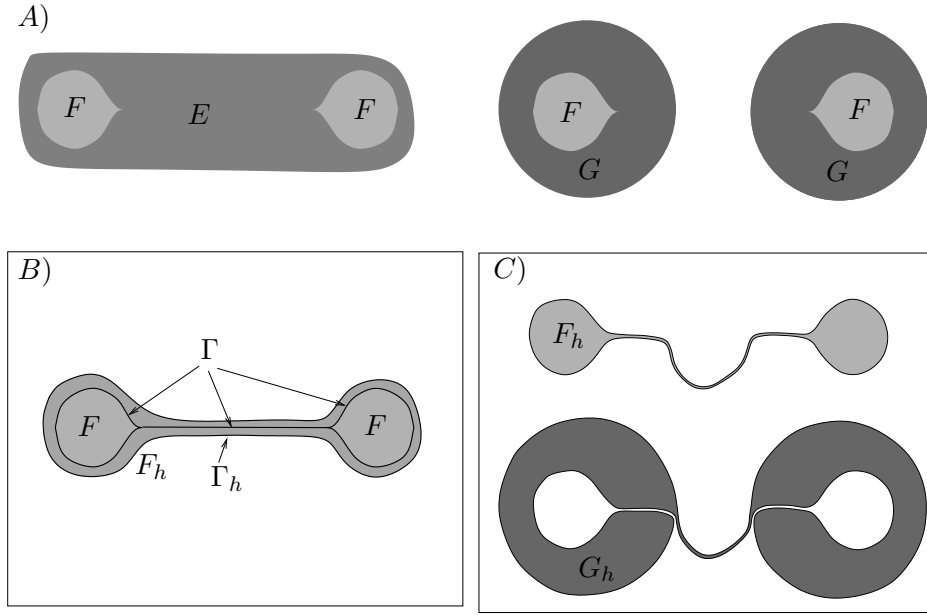
Figure 2.1: Situations of accumulation
