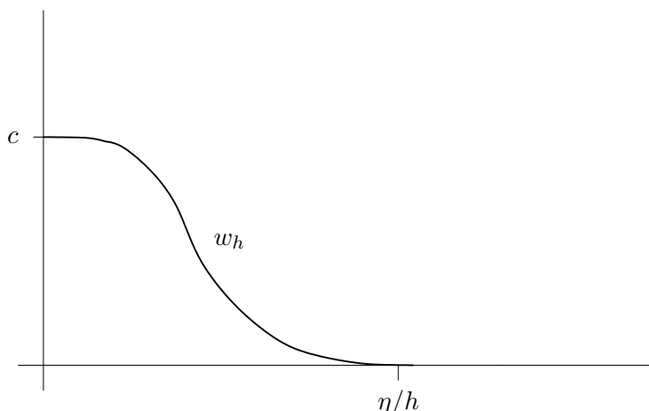
Figure 3.1: Graph of the cut-off function w_h
