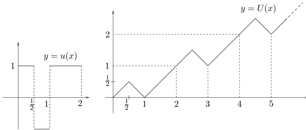
Figure 1.4: Graphs of the functions u and U
