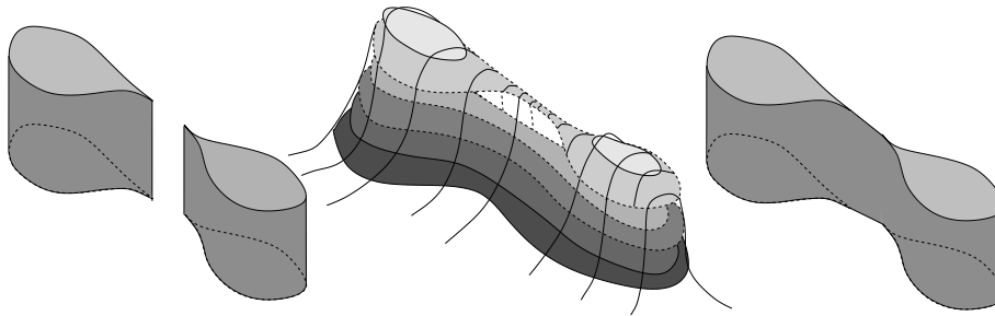
Figure 1.1: Left, the characteristic function of a set of finite perimeter. Middle, an approximating smooth function and some of its level sets. Right, the pointwise limit of a sequence of such approximating smooth functions with uniformly bounded elastica energy.
