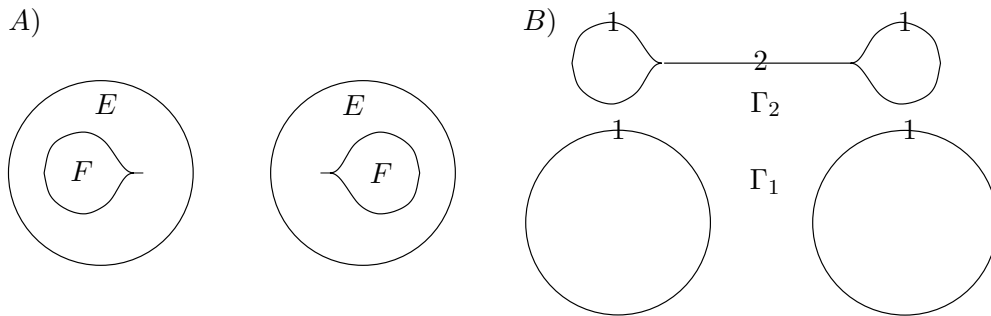
Figure 3.3: If u = \mathbb{1}_{E \cup F} + \mathbb{1}_F , \overline{F}(u) does not coincide with the integral of \overline{W}(\{u > t\}) .
