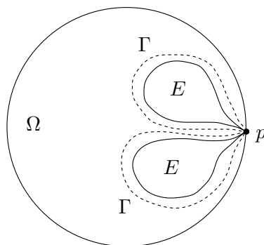
Figure 4.2: L(\mathbf{1}_E, \Omega) = \infty but \overline{F}_B(\mathbf{1}_E, \Omega) < \infty
