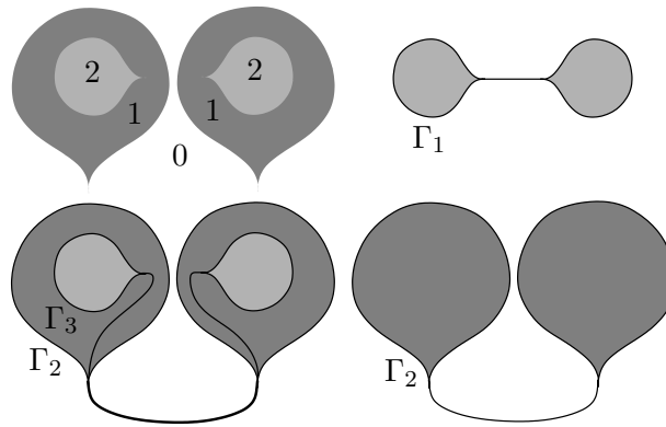
Figure 1.2: The piecewise constant function u on the top left figure has energy \overline{F} strictly greater than \int_{\mathbb{R}} \overline{W}(\{u > t\})dt . Considering an approximating sequence of smooth functions for \mathbb{1}_{\{u \geq 2\}} , the pointwise singular limit is the bold curve \Gamma_1 shown in the top right figure, according to Theorem 8.6 in [5]. The singular limit yielded by the approximation of \mathbb{1}_{\{u \geq 1\}} is (approximately) the curve \Gamma_2 shown in the bottom right figure. Instead, the smooth approximation of u yields as pointwise singular limit the two curves \Gamma_2 and \Gamma_3 roughly represented in the bottom left figure. One has \overline{F}(u) = W(\Gamma_2) + W(\Gamma_3) > W(\Gamma_1) + W(\Gamma_2) = \int_{\mathbb{R}} \overline{W}(\{u > t\})dt .
