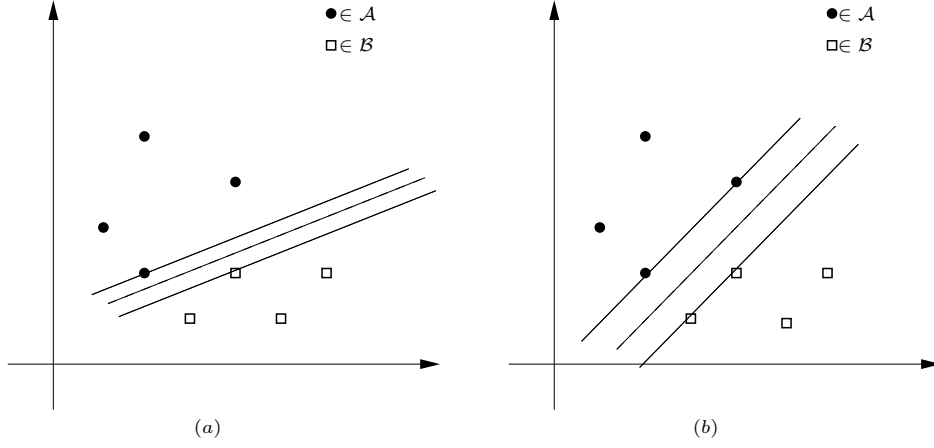
Figure 5.1: (a) A separating hyperplane. (b) A robust separating hyperplane.
