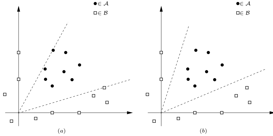
Figure 5.2: (a) An homogeneous separator. (b) The most robust homogeneous separator.
