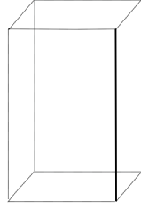
Figure 5.2: Choosing F as a the vertical load F = (0, 0, \sqrt{Y}/12(x_1 - x_2) + \sqrt{Y}) , namely as in Example 3.6 with a_1 = b = \sqrt{Y} and a_2 = -\sqrt{Y} , it turns out that a particular solution of problem (42) is \bar{\mu} = \mathcal{H}^1|_{\{1\} \times \{-1\} \times [-1/2, 1/2]} .
