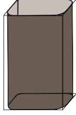
Figure 5.3: Choosing F as the vertical load F = (G_1, G_2, 0) , being G_\alpha as in Example 3.7 such that m_G = (\delta_{-1/2} - \delta_{1/2}) , the optimal measure \bar{\mu} of problem (42) turns out to be concentrated, section by section, on the boundary of the Cheeger set of the section D (here, a square).
