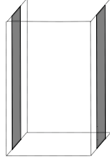
Figure 5.1: Choosing F as a the vertical load F = (0, 0, -\sqrt{Y}/12 x_1) , namely as in Example 3.6 with a_2 = b = 0 and a_1 = -\sqrt{Y} , it turns out that a particular solution of problem (42) is \bar{\mu} = \mathcal{H}^2 \llbracket_{\{\pm 1\} \times [-1/4, 1/4] \times [-1/2, 1/2]} .
