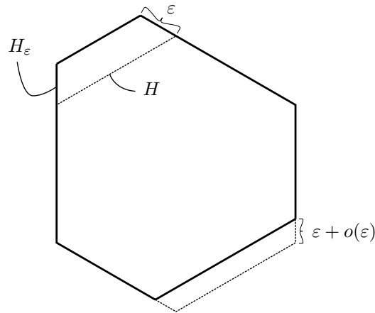
Figure 1.2: We choose a small perturbation of the regular hexagon H in an area-fixing way. Some easy calculations show that h(H_\varepsilon) - h(H) \approx c_0 A(\varepsilon)^2 = c_1 |H_\varepsilon \Delta H|^2 \approx c_2 \text{hd}(\partial H_\varepsilon, \partial H)^2 , where A(\varepsilon) denotes the areas bounded by the dotted lines. Thus yields the sharpness of (6) and (7).
