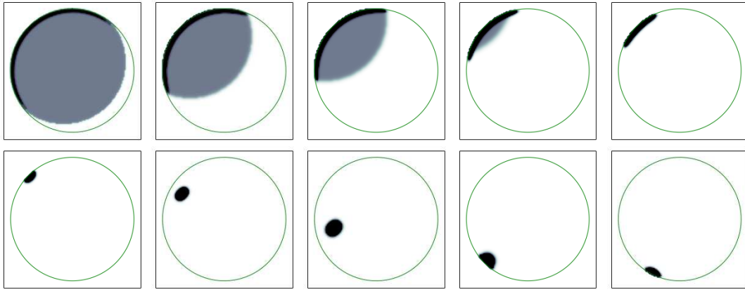
Figure 6.5: Catching up with diffusion, \kappa = 1.e - 4 , at times 1, 4, 6, 9, 12, 24, 26, 30, 34, 38.
