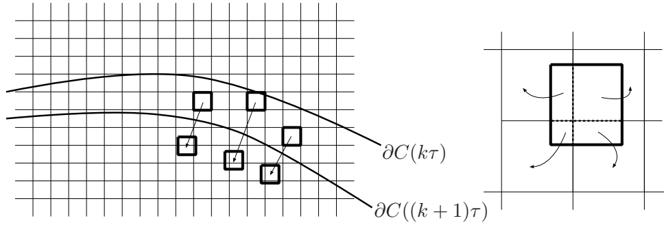
Figure 6.1: Catching-up at the discrete level
