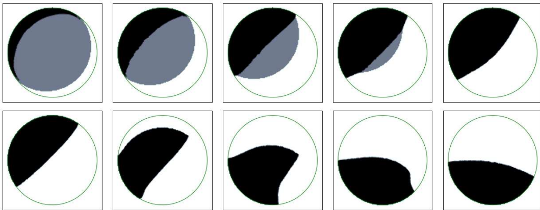
Figure 6.6: Catching up with congestion, at times 1, 2, 3, 4, 5, 24, 26, 29, 32, 35.
