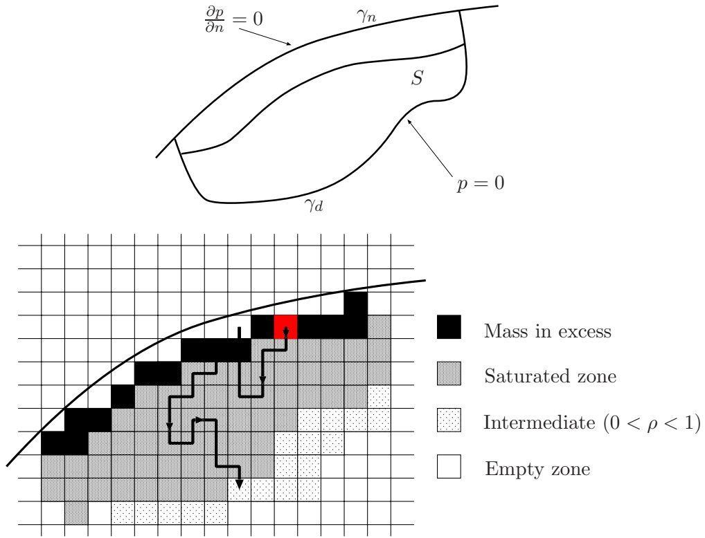
Figure 6.2: Stochastic algorithm
