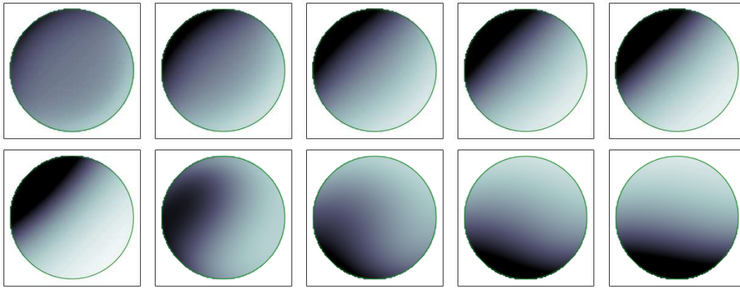
Figure 6.4: Catching up with diffusion, \kappa = 0.1 , at times 1, 2, 3, 4, 5, 24, 26, 28, 30, 32.
