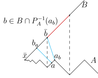
Figure 2.1: BLPW-DIL-restricted regularity but not DIL-restricted regularity
