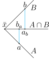
Figure 2.2: DIL-restricted regularity but not BLPW-DIL-restricted regularity
