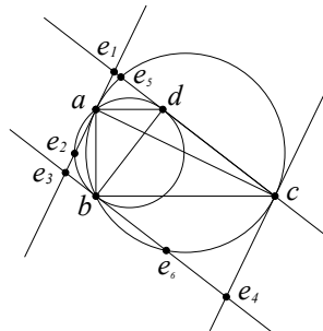
Figure 13: F_1 is of type 4-3, e \in W_{ac} \cap W_{bd}
