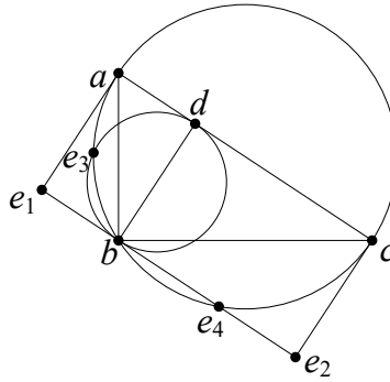
Figure 9: F_1 is of type 4-1, e \in W_{ac} \cap W_{bd}
