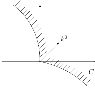
Figure 3.2: A nonconvex set C satisfies assumptions (A1) and (A3).
