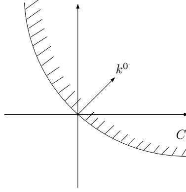
Figure 3.1: A convex set C satisfies assumptions (A1) and (A3).
