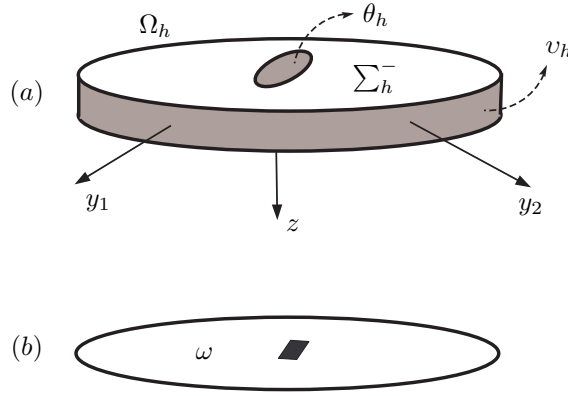
Figure 1.1: A plate with small clamped area (a) and its two-dimensional model where the black square indicates an asymptotic point condition (b).
