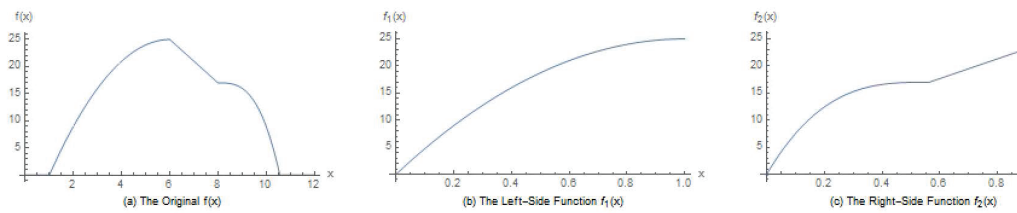
Figure 3.1: The Construction of f_1 and f_2 .
