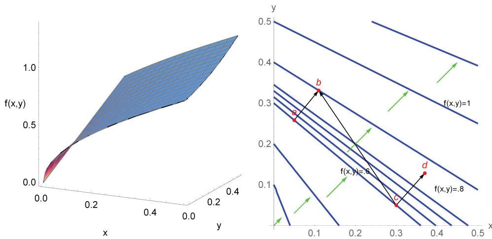
Figure 2.1: Fenchel's Example: Nonconcavifiable with Linear Level Sets.
