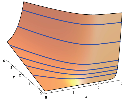
Figure 5.1: A function violating condition (iii) of Theorem 5.1 and some level sets.
