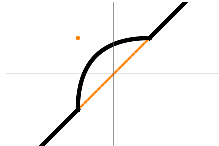
Figure 3.4: Monotone Hull
