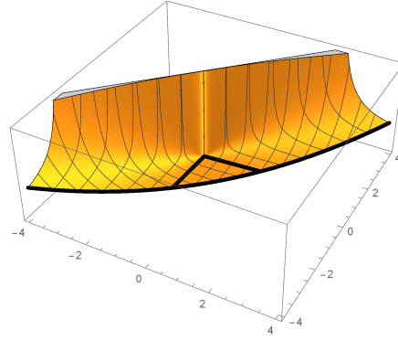
Figure 3.2: \sigma_\Gamma
