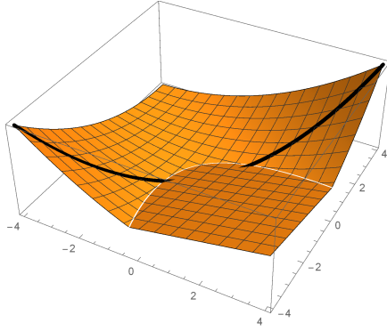
Figure 3.1: \varphi_\Gamma
