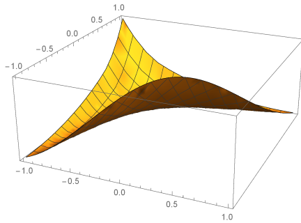
Figure 3.3: h_\Gamma - \pi
