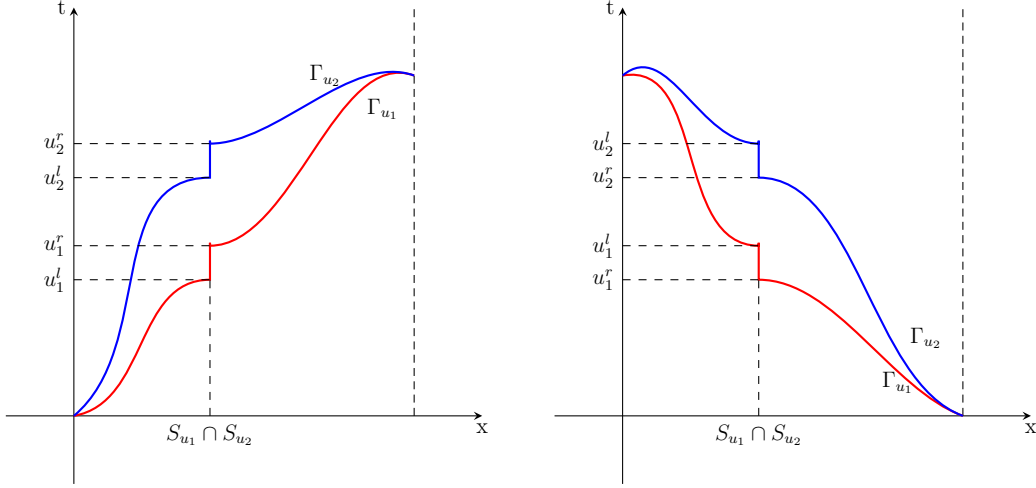
Figure 3.2: Configuration in Lemma 3.12 and in Lemma 3.13
