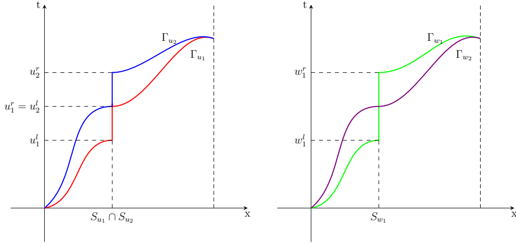
Figure 3.3: Convex decomposition of two SBV graphs
