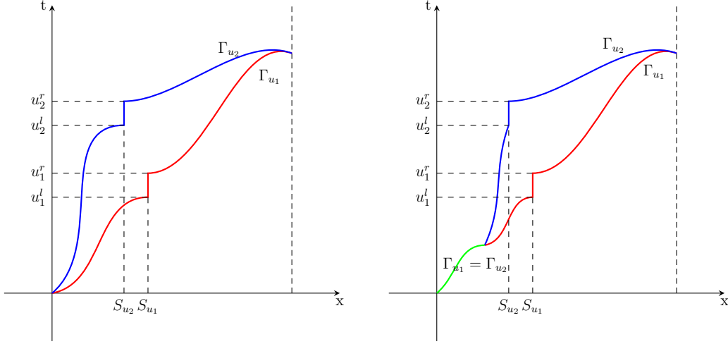
Figure 3.1: Configuration in Lemma 3.8 and 3.9
