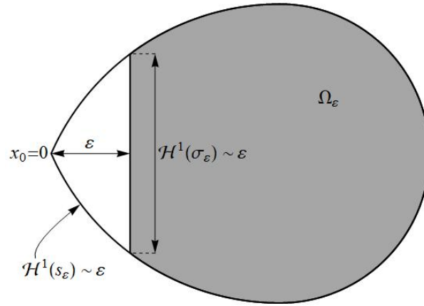
Figure 4.1: Cutting procedure in dimension d = 2 .
