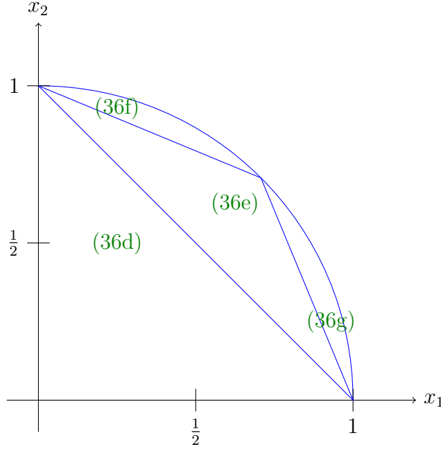
Figure 4.2: Companion figure for Proposition 4.3
