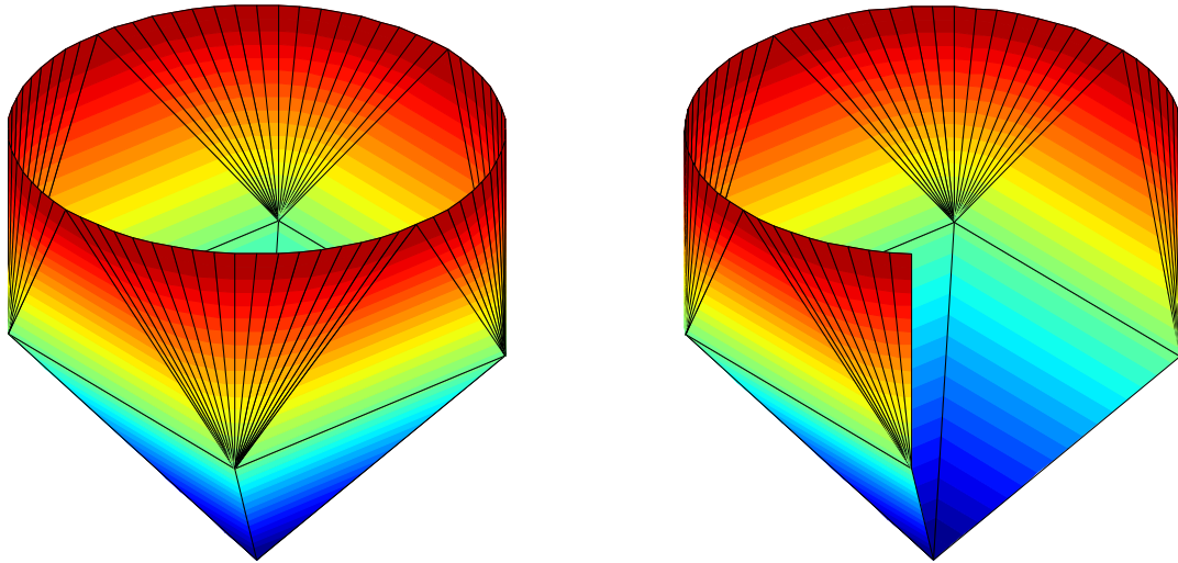
Figure 4.1: Topological closure of the graph, between heights z = 0 and z = 2 , of the proper convex lsc function \mathcal{L}_0 which coincides, on the Euclidean unit sphere \mathbb{S} , with the \ell_0 pseudonorm
