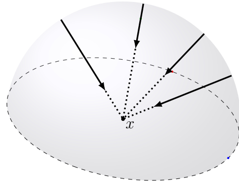
Figure 2. An affine hemisphere of elliptic type in \mathbb{R}^3
