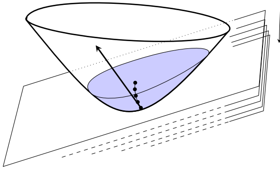
Figure 1. Geometrical construction of the affine normal.
