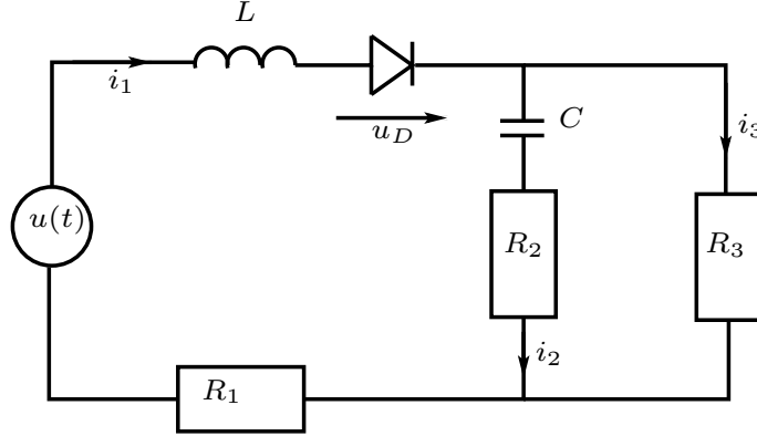
Figure 6.1: An RLCD passive circuit.
