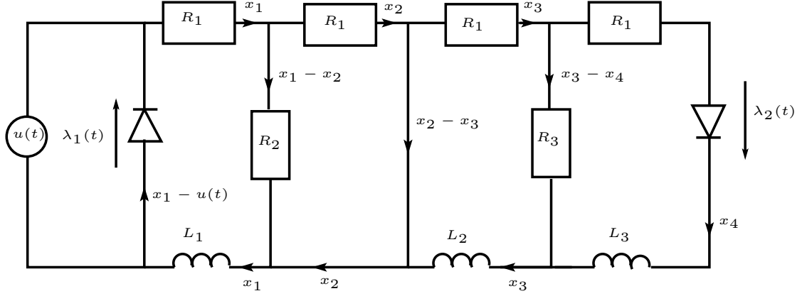
Figure 6.3: An RLCD passive circuit.
