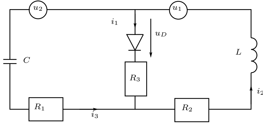
Figure 6.2: An RLCD passive circuit.
