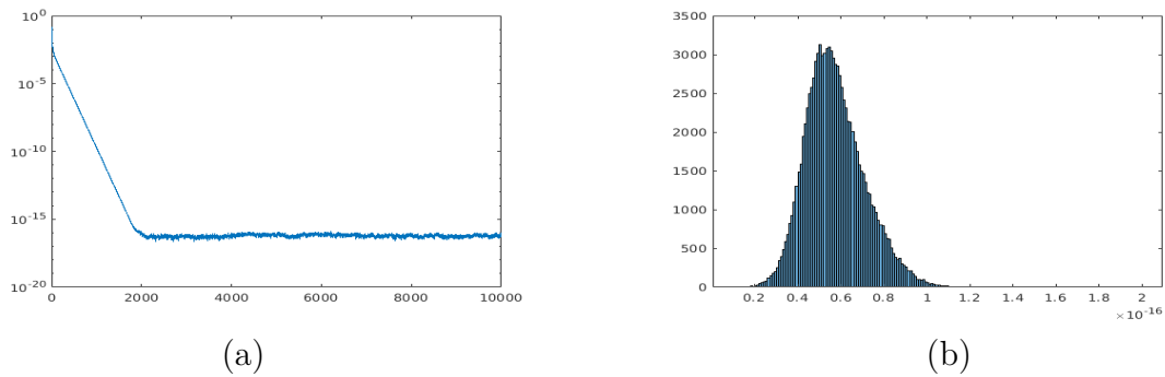
Figure 1.1: (a) The residual x_{k+1} - x_k of iterates of the cyclic projections algorithm for solving the linear system Ax = b for A \in \mathbb{R}^{50 \times 60} , and b \in \mathbb{R}^{50} randomly generated. (b) A histogram of the residual sizes over the last 8000 iterations.
