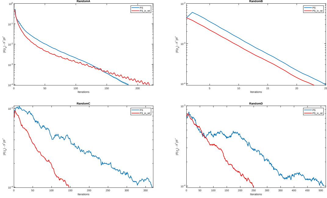
Figure 4: Comparison of performances in LASSO problems
