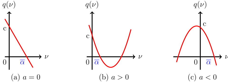
Figure A.1: Possible cases for the real function q(\cdot) in Lemma A.4.
