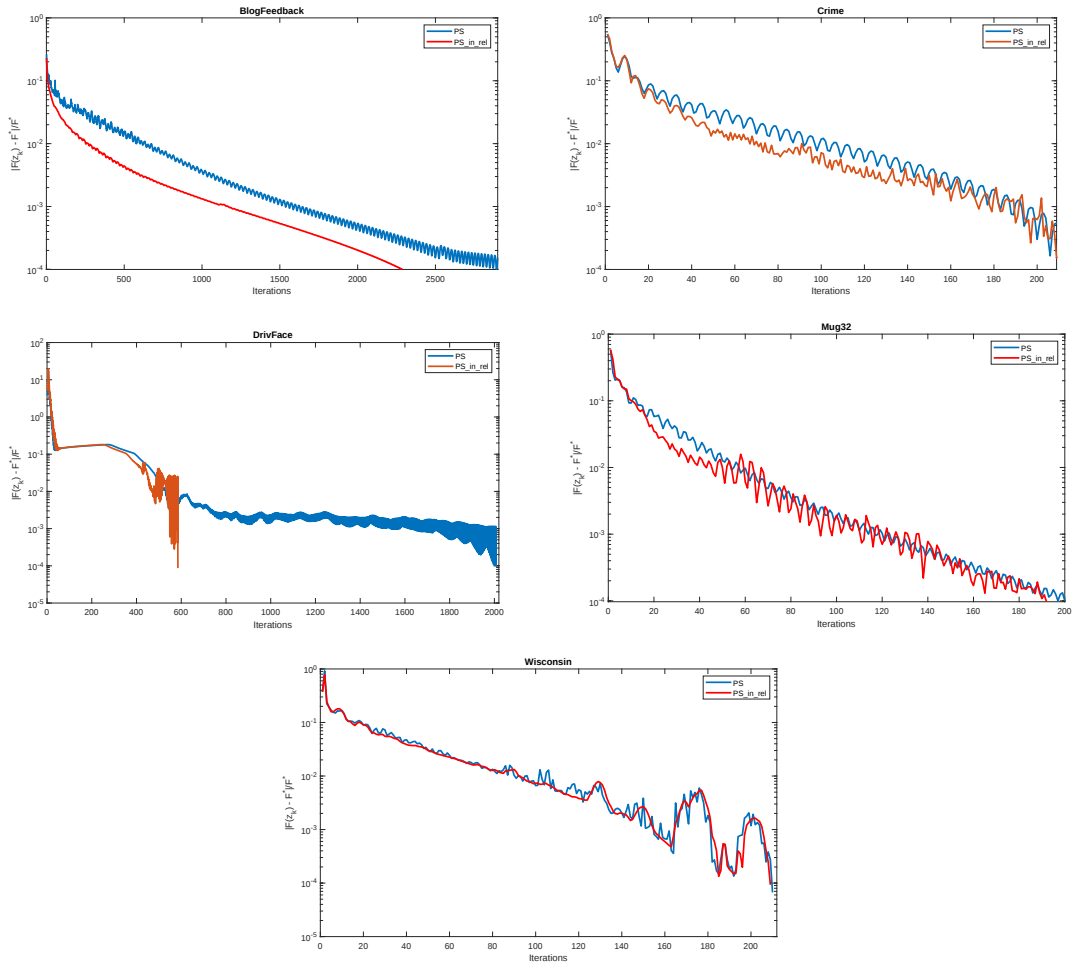
Figure 3: Comparison of performances in LASSO problems
