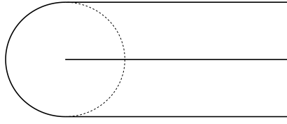
Figure 1.2: The set \mathbf{H} : it can be built by taking the disk \{(x_1, x_2) : x_1^2 + x_2^2 < 1\} , removing the segment [0, 1] \times \{0\} and then adding two parallel half-strips.
