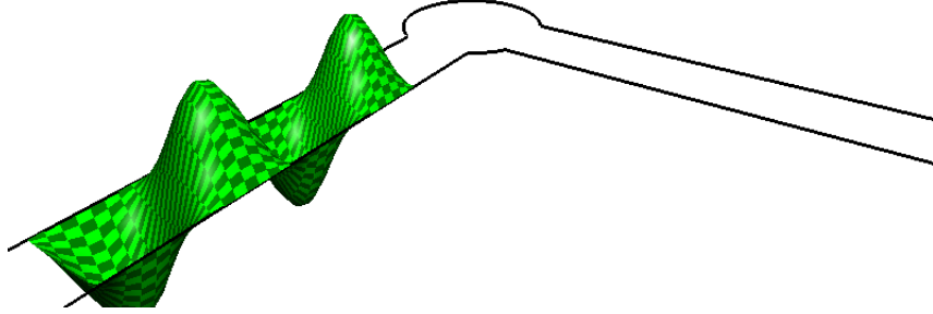
Figure 6.1: The construction of the sequence \varphi_n in the proof of Proposition 6.1.
