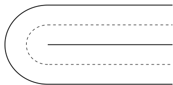
Figure 1.3: In dashed line, the image of the curve \gamma defined by (7). By taking its tubular neighborhood of width 1/2 , we get the set \mathbf{H} .
