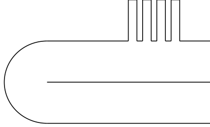
Figure 7.1: The construction of \mathbf{H}_n^\varepsilon , with n = 3 : we add to \mathbf{H} an array of n + 1 = 4 equally spaced vertical tubes. Each tube has height 1 and width 2\varepsilon , with \varepsilon \ll 1 .
