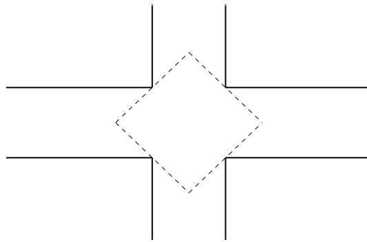
Figure 3.1: The set of Example 3.6. In dashed line, the square Q having the property \lambda_1(Q) \leq \mathcal{E}(\Omega) .
