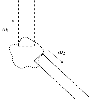
Figure 1.1: An example of a set verifying Assumptions 1.2, in dimension N = 2 and with k = 2 disjoint tubes \mathcal{C}_1 and \mathcal{C}_2 .
