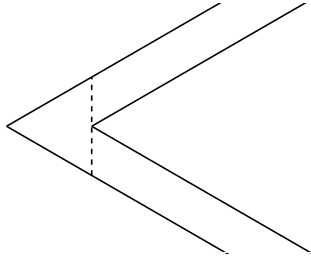
Figure 3.2: The set of Example 3.7. In dashed line, the triangle T having the property \lambda_1(T) \leq \mathcal{E}(\Omega) .
