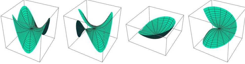
Figure 2.2: Graphs of f_1^1, f_1^2, f_1^3, f_1^4 , exhibiting resp. crease, jump, crease, jump.
