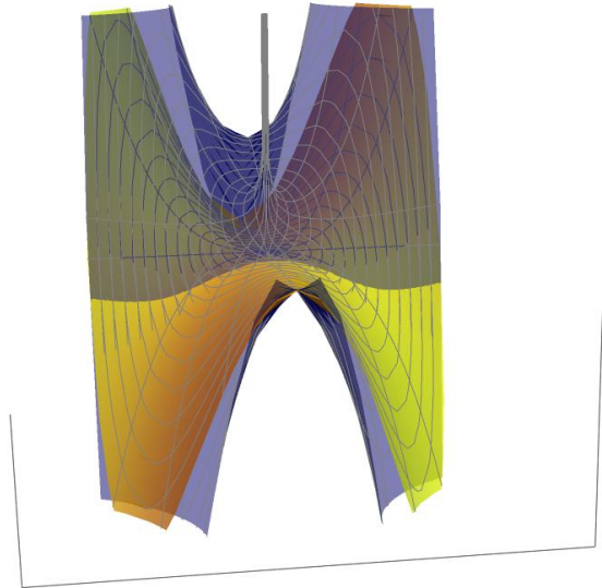
Figure 4.1: An approximation in L^2(B_\varrho) (blue graph: first 100 terms in the series) of w = r^3(\cos(\vartheta) - \cos(3\vartheta)) matching the function w itself (yellow graph).
