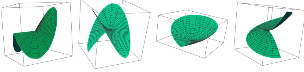
Figure 2.1: Graphs of f_0^1, f_0^2, f_0^3, f_0^4 , exhibiting resp. crease, jump, crease, jump.
