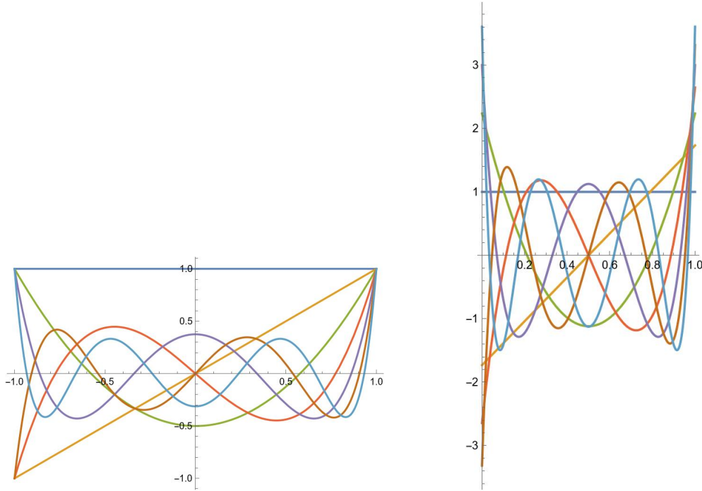
Figure 2.3: Graphs of Legendre polynomials P_n in L^2(-1, 1) (left) and graphs of rescaled and normalized shifted Legendre polynomials \tilde{P}_n in L^2(0, 1) (right), n = 0, 1, 2, 3, 4, 5, 6 .
