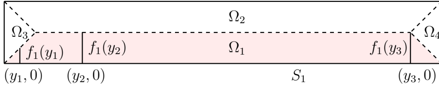
Figure 3.1: The partition of \Omega = (-\frac{L}{2}, \frac{L}{2}) \times (0, 1) , when L > 1 , by means of the sets \Omega_i , and the function f_1 = f_1(y) with (y, 0) \in S_1 . We note that f_1(y_3) = 1/2 = L/2 - y_3 .
