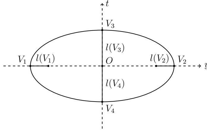
Figure 4.1: The values l(V_i) where V_i are the vertices of the ellipse with equation
