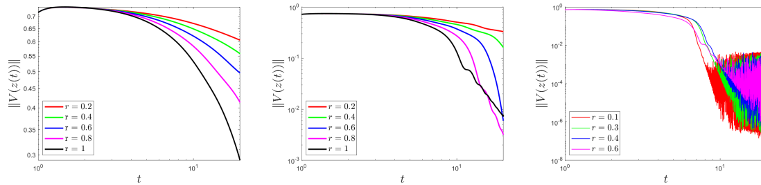
Figure 2.3: Influence of r on the norm of the operator along the trajectories, with parameter \beta chosen respectively as \beta(t) \equiv 1 , \beta(t) = t and \beta(t) = \frac{1}{t^{2r}} \exp \left[ \left( \frac{1}{\theta} - \delta \right) \frac{t^{1-r}}{1-r} \right]
