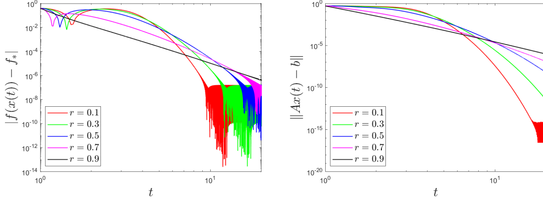
Figure 2.2: Influence of r on the functional values and feasibility gap along the trajectories, \beta(t) = \frac{1}{t^{2r}} \exp \left[ \left( \frac{1}{\theta} - \delta \right) \frac{t^{1-r}}{1-r} \right]
