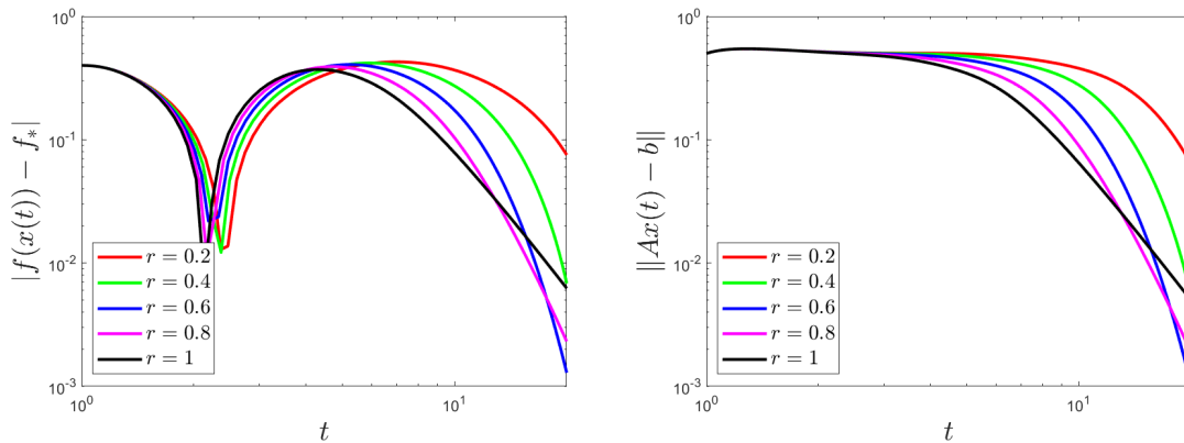
Figure 2.1: Influence of r on the functional values and feasibility gap along the trajectories, \beta(t) \equiv 1
