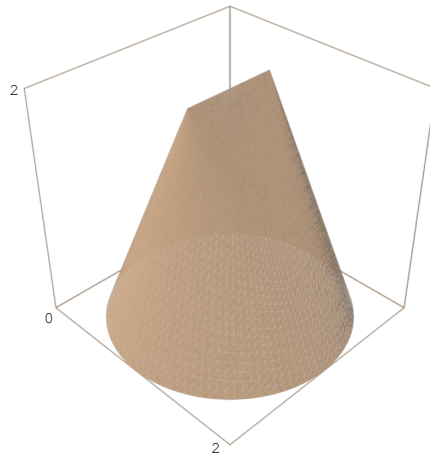
Figure 2. Optimal convex shape with R = 1 and M = 2 .
