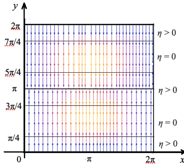
Figure 2. The drift vector field of (11) and the function \eta
