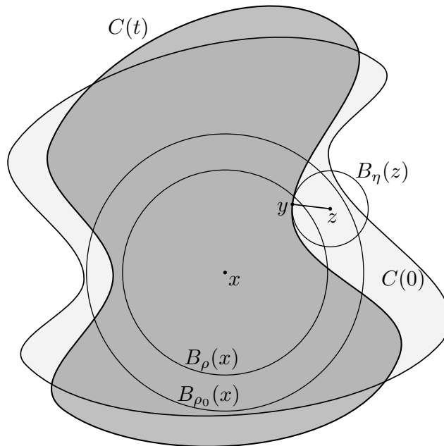
Figure 1. Visual aid for the proof of Lemma 4.6.
